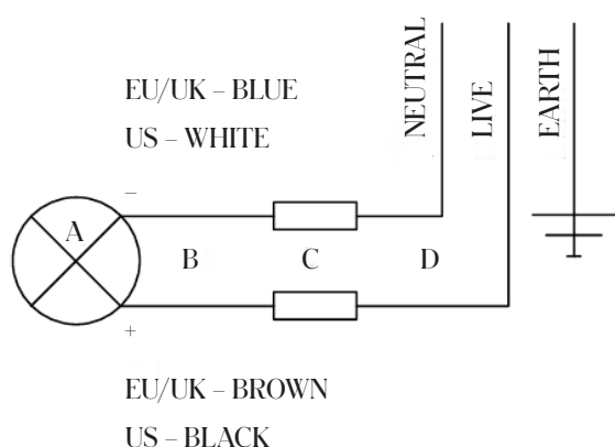
Wiring diagram
